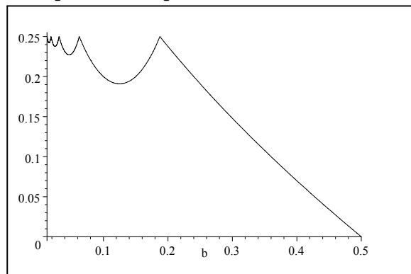
Figure 1: Optimal s^*
